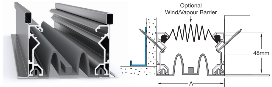
Illustrated: VL-75
