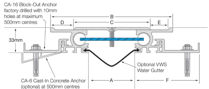
CA-35 - CA-135
