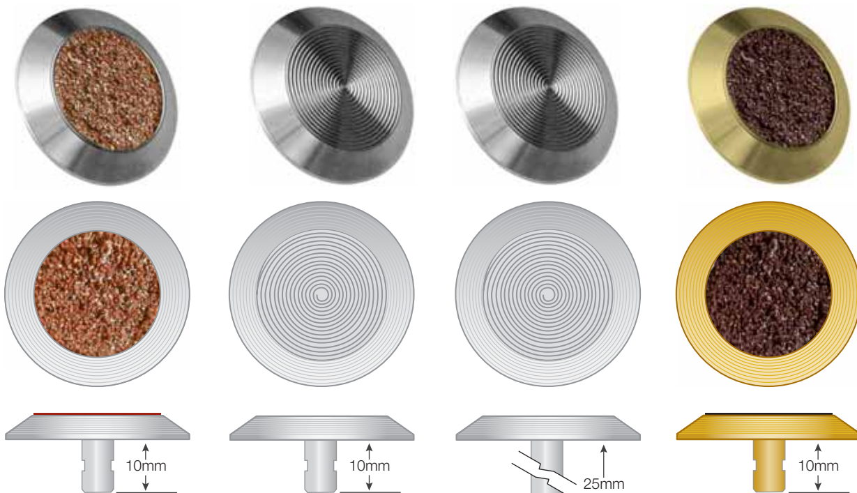
LTAS Tactile Indicator Stud Latham Slip Resistant Abrasive Stainless Steel Tactile Indicator Stud, with Supagrit™ teak silicon carbide mineral insert.
